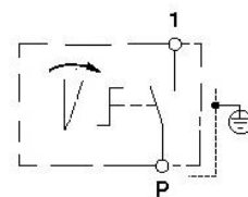
Surface-mount key switch With phc Art.: 009.1101.10
